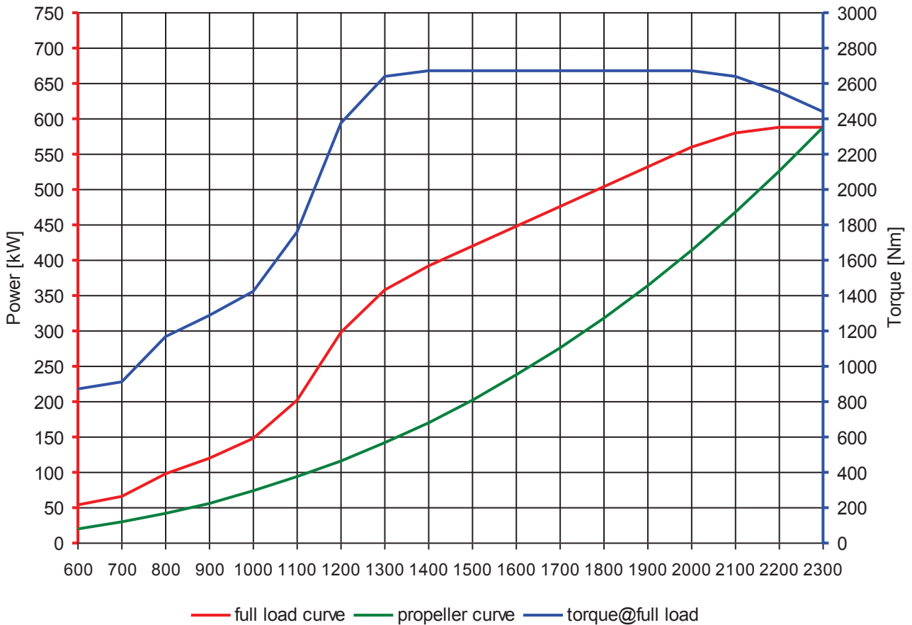
Power/torque curves
